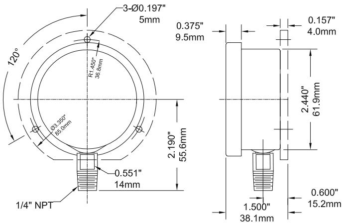
2.5" Bottom Connection with Back Flange
