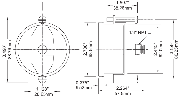
2.5" Back Connection with U-Clamp
