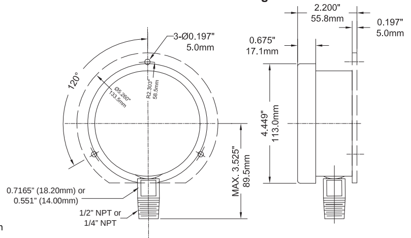
4" Bottom Connection with Back Flange
