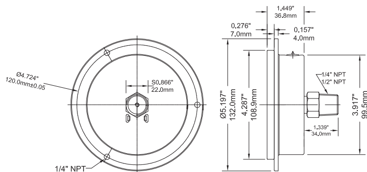
4" Back Connection with Front Flange
