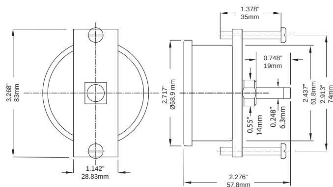
2.5" Back Connection with U-Clamp
