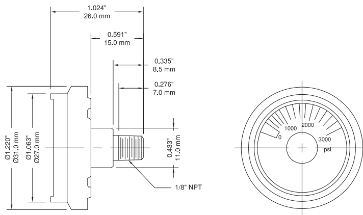
1.25" Spiral Tube Gauge
