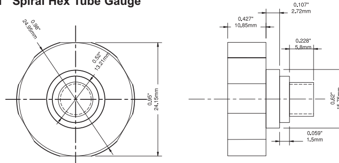
1 1/8" Spiral Tube Gauge
