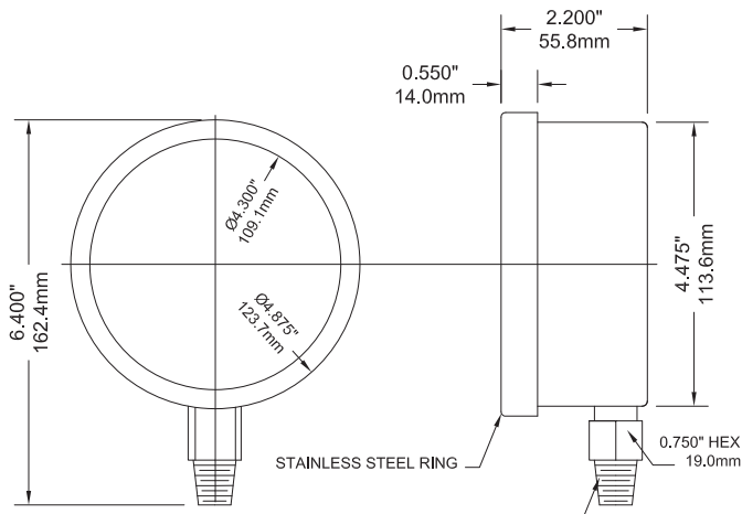
4.5" Bottom Connection Stainless Steel
