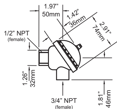
Aluminum Head
