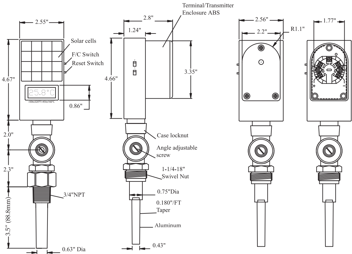
With Thermowell
