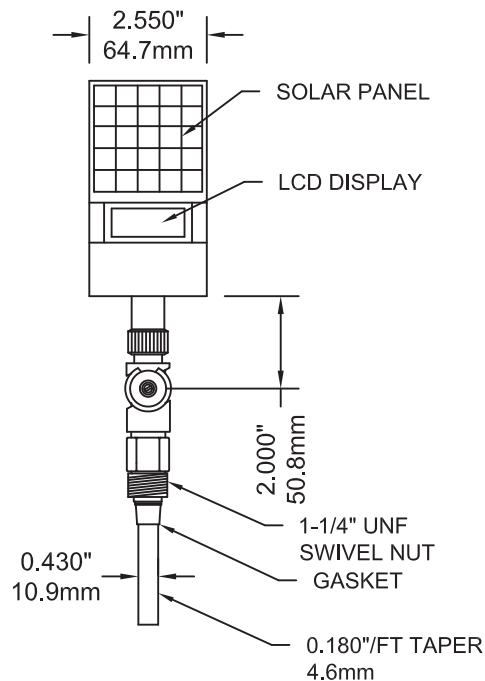
3.5" Stem without Thermowell
