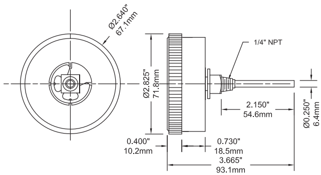
2.5" Back Connection
