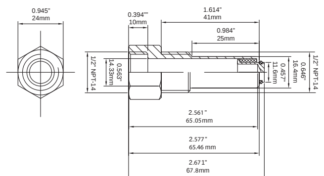
0.5" Brass Thermowell
