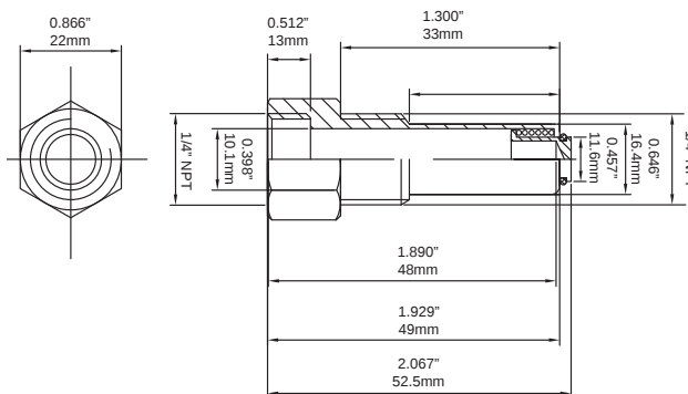
0.25" Brass Thermowell
