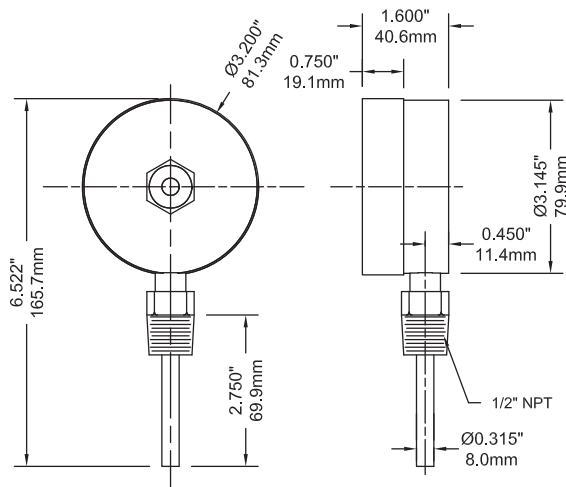
3" Bottom Connection
