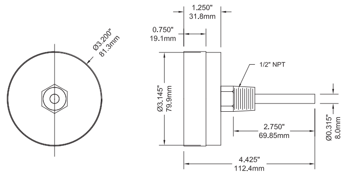
3" Back Connection
