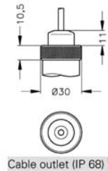
Cable outlet (IP 68)
