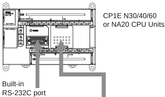
Optional Serial Communication Board
